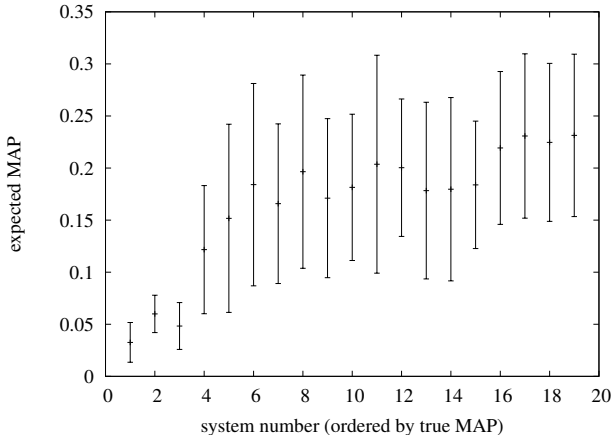
Figure 1: Example 1: one site submitted runs that contributed to a pool of depth 10. These judgments are used to rank 19 new systems from five sites by expected MAP, and to calculate confidence intervals.
