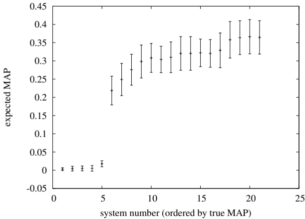
Figure 3: Example 2: three sites submitted runs that contributed to a pool of depth 10. The resulting confidence intervals on new runs are tighter than those in Figure 1.
