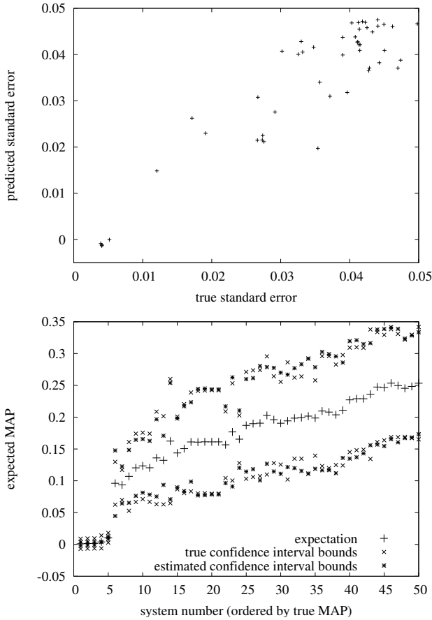
Figure 2: Standard error prediction (top) and expected MAP with both “true” confidence intervals and predicted confidence intervals (bottom) for testing systems.
